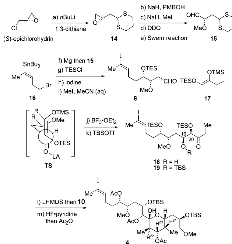
Scheme 2. Reagents: (a) 1,3-dithiane, n BuLi, THF, -40\text{ }^{\circ}\text{C} to room temp. (76%). (b) NaH, PMBOH, DMF, 50\text{ }^{\circ}\text{C} (69%). (c) MeI, NaH, THF, 0\text{ }^{\circ}\text{C} (95%). (d) DDQ, \text{CH}_2\text{Cl}_2/\text{H}_2\text{O} (4:1), 0\text{ }^{\circ}\text{C} (75%). (e) (\text{COCl})_2 , DMSO, \text{Et}_3\text{N} , \text{CH}_2\text{Cl}_2 , -78\text{ }^{\circ}\text{C} to 0\text{ }^{\circ}\text{C} (81%). (f) 15 , Mg, 1,2-dibromoethane, \text{Et}_2\text{O} , -78\text{ }^{\circ}\text{C} (60–70%). (g) TESCl, imid., \text{CH}_2\text{Cl}_2 , room temp. (h) \text{I}_2 , \text{CH}_2\text{Cl}_2 , 0\text{ }^{\circ}\text{C} (90%, two steps). (i) MeI, \text{K}_2\text{CO}_3 , MeCN/pH 7 buffer (4:1), 28\text{ }^{\circ}\text{C} (75%). (j) \text{BF}_3\cdot\text{OEt}_2 , \text{CaH}_2 , \text{CH}_2\text{Cl}_2 , -94\text{ }^{\circ}\text{C} (69%). (k) TBSOTf, 2,6-lutidine, \text{CH}_2\text{Cl}_2 , -78\text{ }^{\circ}\text{C} (93%). (l) LHMDs, HMPA, 10 , THF, -78\text{ }^{\circ}\text{C} (85%). (m) HF \cdot pyr, pyr, THF, room temp. then \text{Ac}_2\text{O} , pyr., room temp. (64%).
