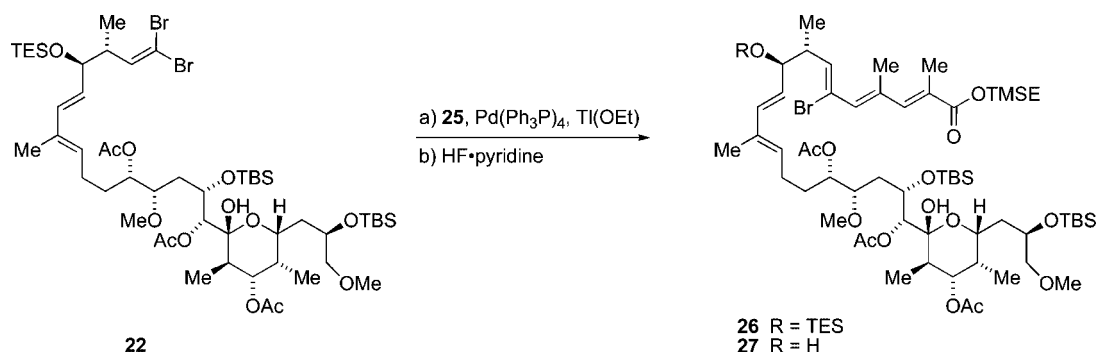
Scheme 4. Reagents: (a) 25 , [\text{Pd}(\text{Ph}_3\text{P})_4] , \text{Ti}(\text{OEt})_4 , \text{THF}/\text{H}_2\text{O} (3:1), room temp. (71%). (b) HF·pyridine, \text{THF} , 0^\circ\text{C} (66%).
