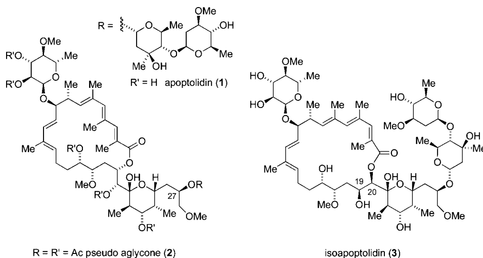
Figure 1. Structure of apoptolidin ( 1 ), pseudo aglycone ( 2 ) and isoapoptolidin ( 3 ).
