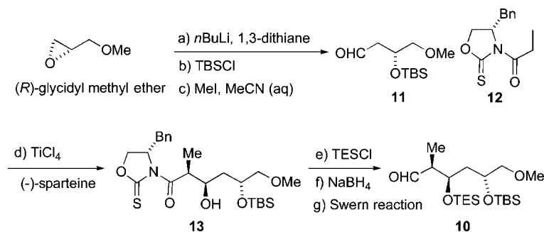
Scheme 1. Reagents; (a) 1,3-dithiane, n BuLi, THF, -40^{\circ}\text{C} (90–95%). (b) TBSCl, ImH, \text{CH}_2\text{Cl}_2 , room temp. (90–95%). (c) MeI, \text{K}_2\text{CO}_3 , MeCN/ \text{H}_2\text{O} (10:1), 40^{\circ}\text{C} (90%). (d) \text{TiCl}_4 , (–)-sparteine, \text{CH}_2\text{Cl}_2 , -78^{\circ}\text{C} (90–95%). (e) TESCl, imid., DMF, 0^{\circ}\text{C} (90–95%). (f) \text{NaBH}_4 , MeOH, room temp. (68%). (g) (\text{COCl})_2 , DMSO, \text{Et}_3\text{N} , \text{CH}_2\text{Cl}_2 , -78^{\circ}\text{C} to 0^{\circ}\text{C} (88%).
