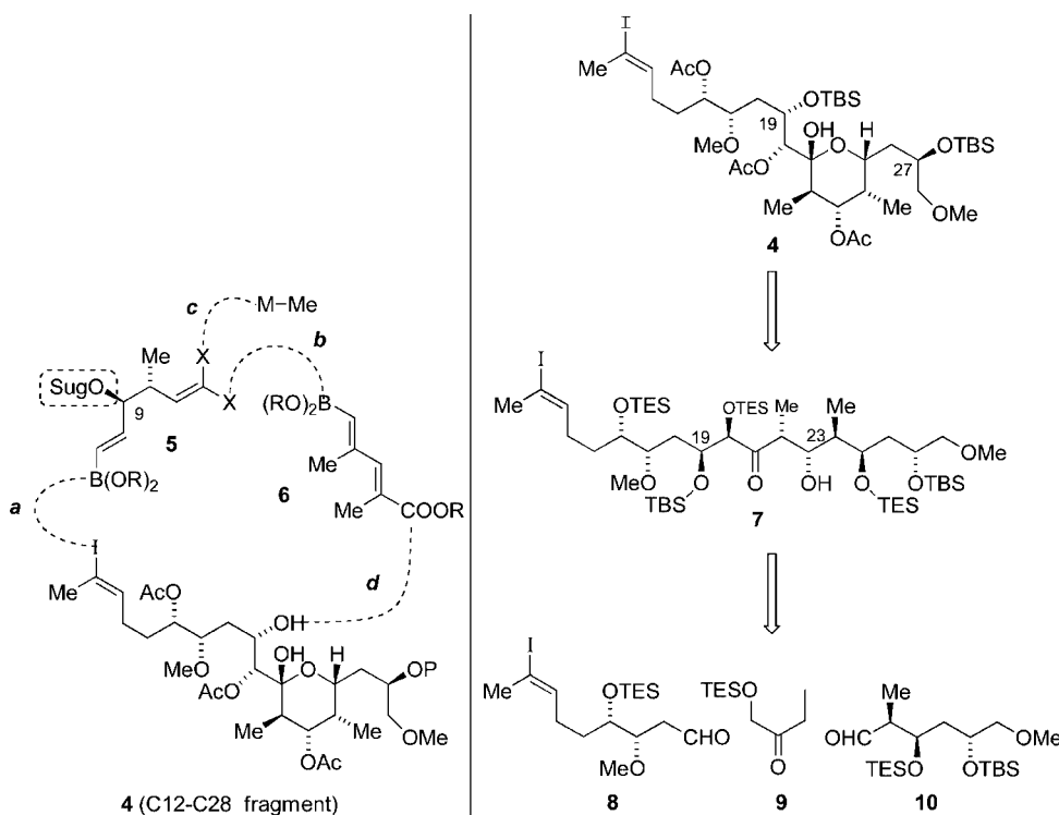
Figure 2. Retrosynthetic analysis of the pseudo aglycone of apoptolidin ( 2 ) and C12–C28 fragment ( 4 ).
