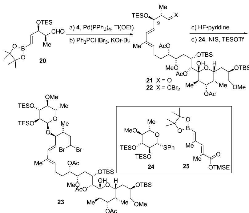
Scheme 3. Reagents: (a) 4 , [\text{Pd}(\text{Ph}_3\text{P})_4] , \text{Ti}(\text{OEt})_4 , \text{THF}/\text{H}_2\text{O} (3:1), room temp. (88%). (b) \text{Ph}_3\text{PCHBr}_3 , \text{KOt-Bu} , \text{THF} , 0^\circ\text{C} (82%). (c) HF·pyridine, \text{THF} , 0^\circ\text{C} (80%). (d) 24 , NIS, TESOTf, \text{CH}_2\text{Cl}_2 , 4-Å molecular sieves, -20^\circ\text{C} (45%).
